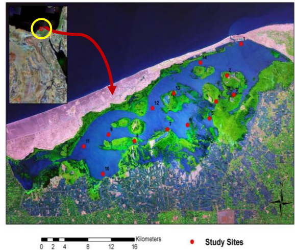
Fig. 1: Satellite map of the study area showing Burullus Lake close to the Mediterranean Sea. Numbered (1-14) red circles are the study sites.
